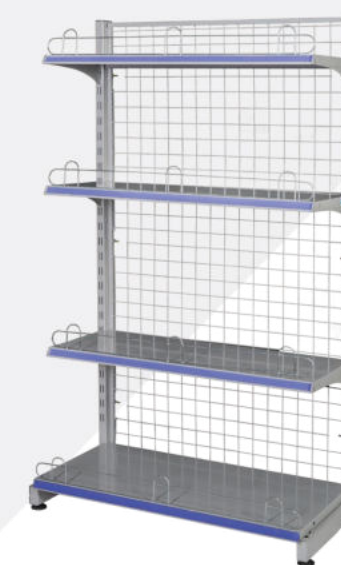
GST02 W900 x D480 x H1500 mm
